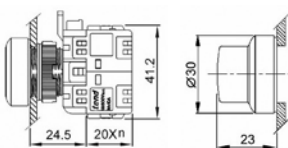
PB22SS Series Push Button
