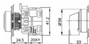
PB22SH Series Push Button
