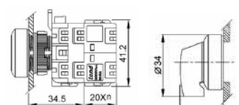
Illuminated PB22IH Series Push Button
