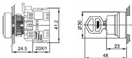
PB22KS Series Push Button
