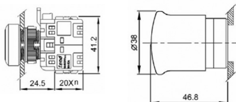
PB22BP Series Push Button
