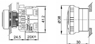
PB22BK Series Push Button
