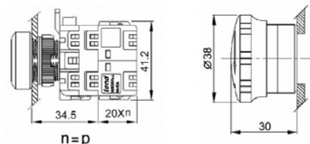
Illuminated PB22IK Series Push Button
