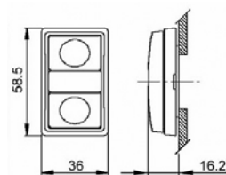
PB22BT Series Push Button
