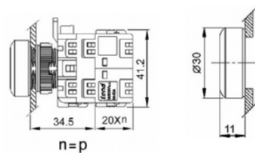
Illuminated PB22IF Series Push Button
