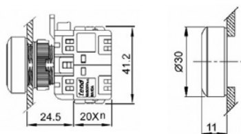
PB22BF Series Push Button
