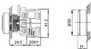
PB22 Series Push Button
