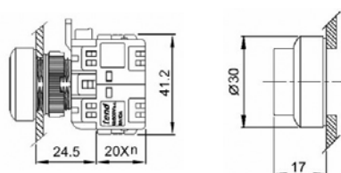
PB22 Series Push Button
