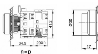
Illuminated PB22 Series Push Button
