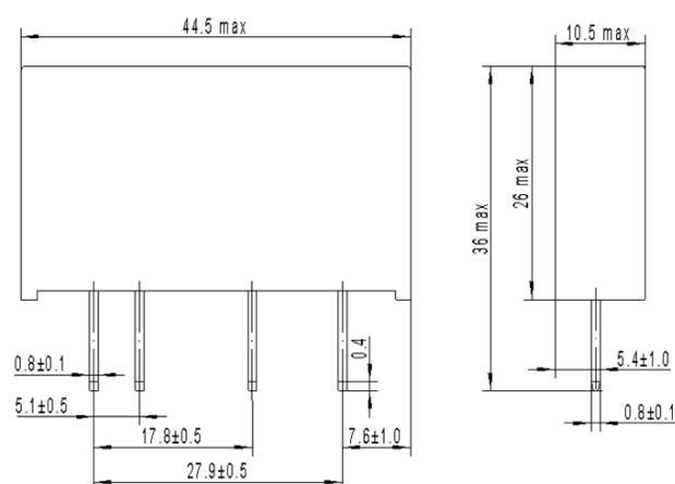
Outline Dimensions
