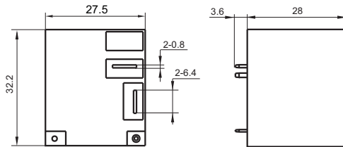
Outline Dimensions
