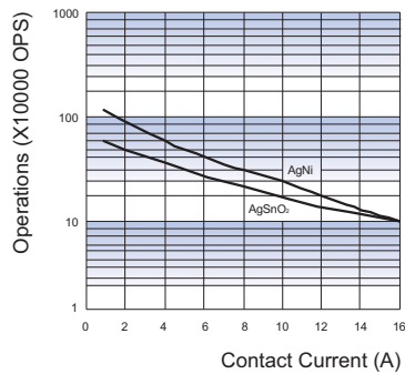
ENDURANCE CURVE
