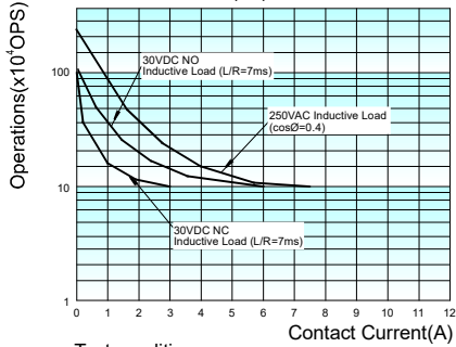
ENDURANCE CURVE (1Z)
