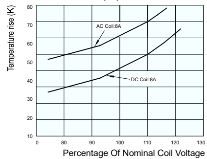
COIL TEMPERATURE RISE (2Z)
