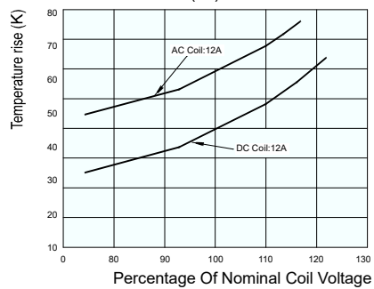
COIL TEMPERATURE RISE (1Z)
