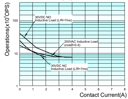
ENDURANCE CURVE (2Z)
