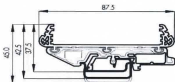
supporto profilato E 72 MT2 (E72CM) con gancio E72G profile support E 72 MT2 (E72CM) with coupling E72CLGL
