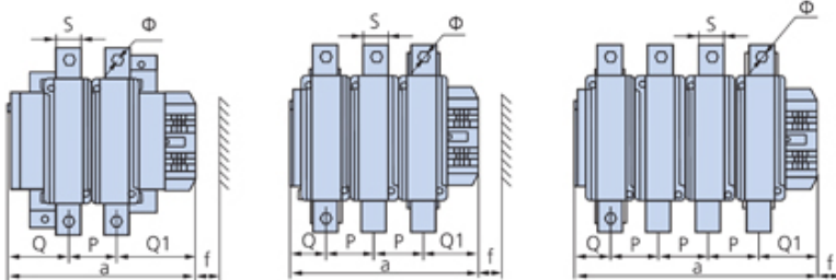
External Dimension
