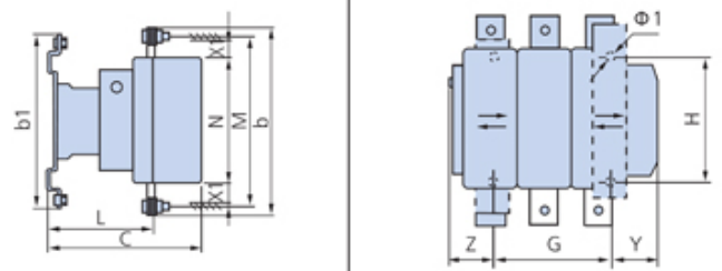
Install size
